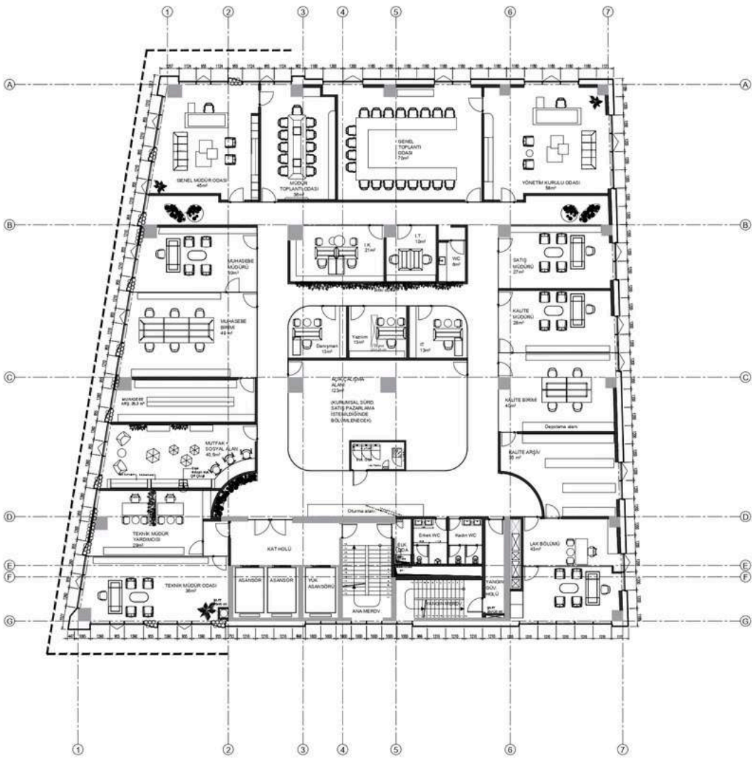
EKOTEKS - 3RD NORMAL FLOOR
