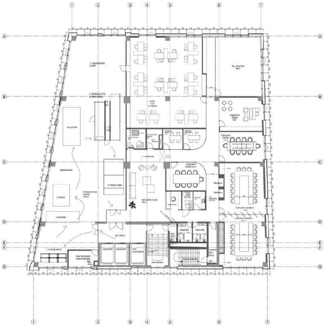
DDM - 4TH NORMAL FLOOR
